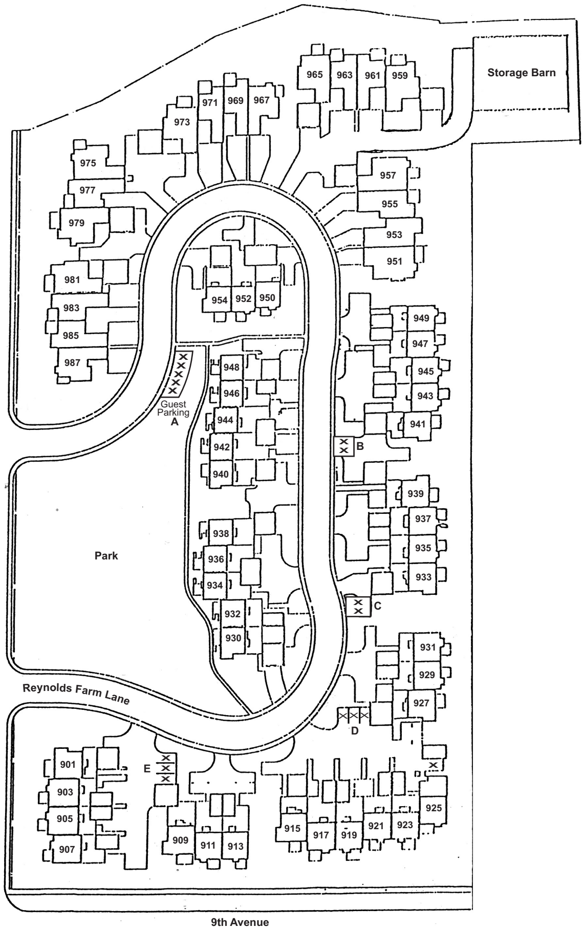
Reynolds Farm Site Plan with 16 Guest Parking Spaces marked with X
